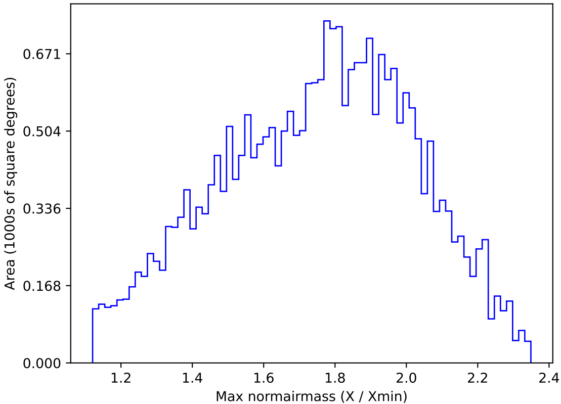
too_elab_r8_d2_giz_v3.4_10yrs All sky g band: Max normairmass
