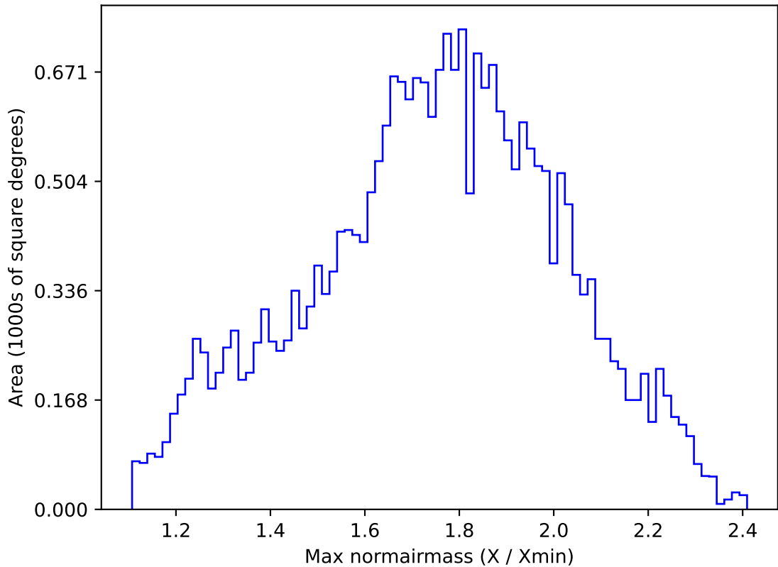
too_elab_r8_d2_giz_v3.4_10yrs All sky g band: Max normairmass
