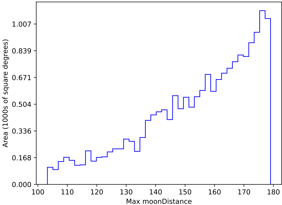
too_elab_r8_d2_giz_v3.4_10yrs WFD z band: Max moonDistance
