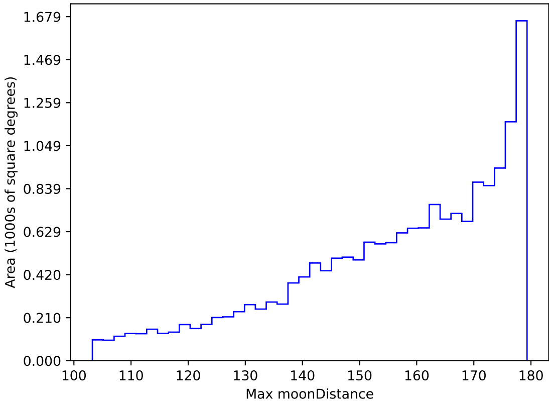
too_elab_r8_d2_giz_v3.4_10yrs WFD r band: Max moonDistance
