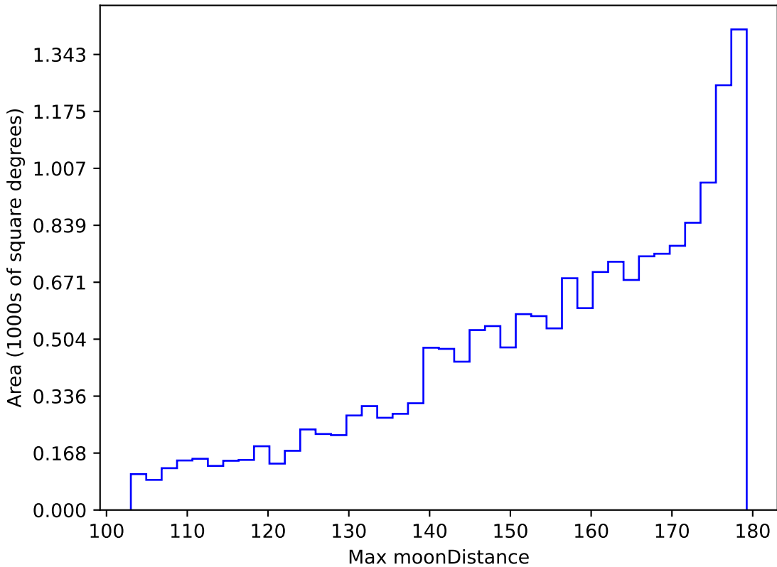
too_elab_r8_d2_giz_v3.4_10yrs WFD i band: Max moonDistance
