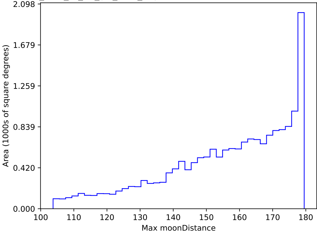
too_elab_r8_d2_giz_v3.4_10yrs WFD all bands: Max moonDistance
