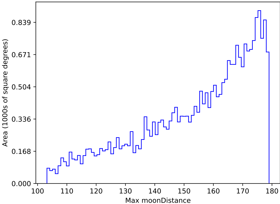
too_elab_r8_d2_giz_v3.4_10yrs All sky z band: Max moonDistance
