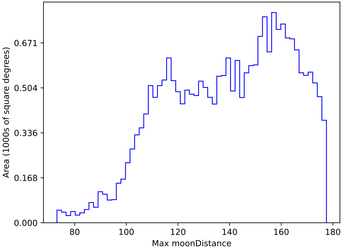
too_elab_r8_d2_giz_v3.4_10yrs All sky y band: Max moonDistance
