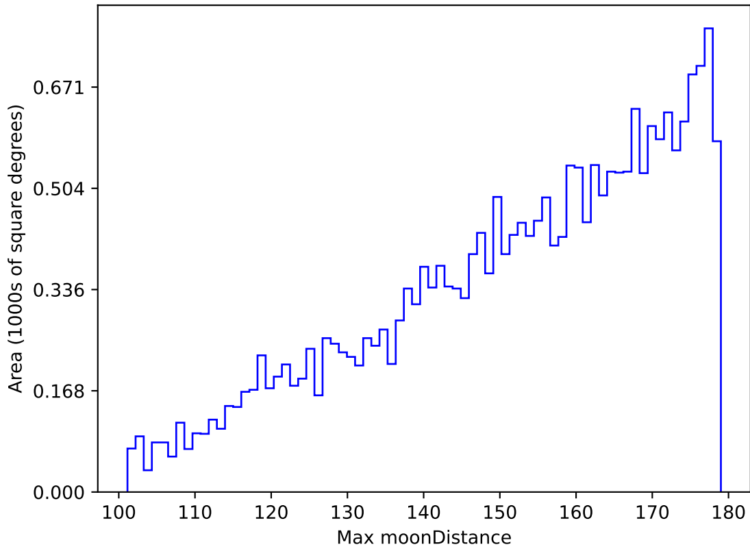
too_elab_r8_d2_giz_v3.4_10yrs All sky u band: Max moonDistance
