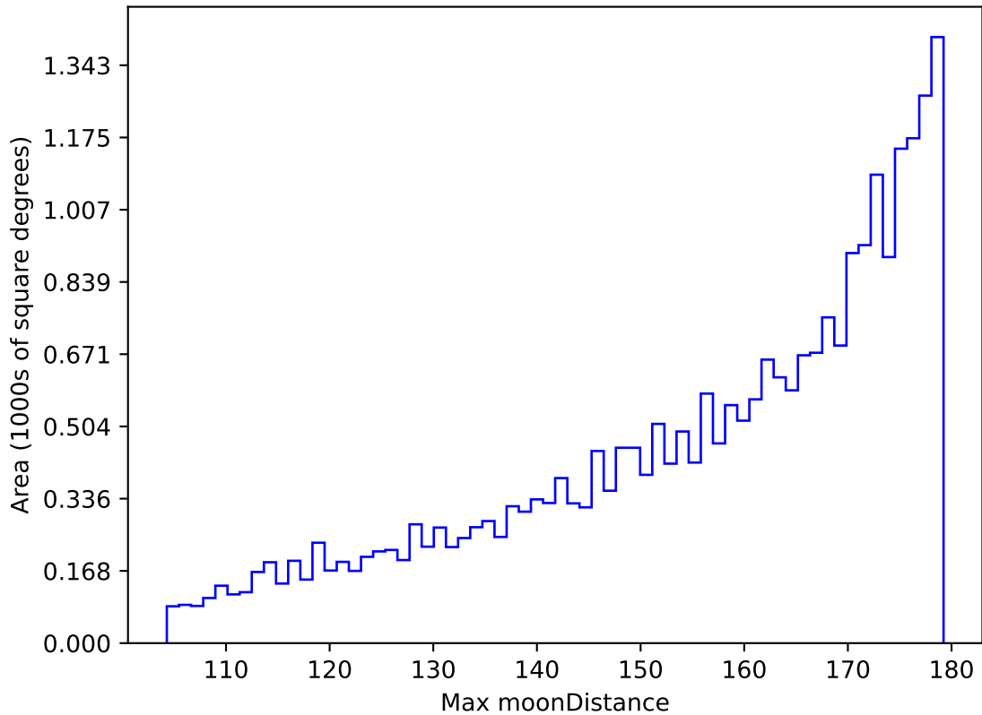
too_elab_r8_d2_giz_v3.4_10yrs All sky r band: Max moonDistance
