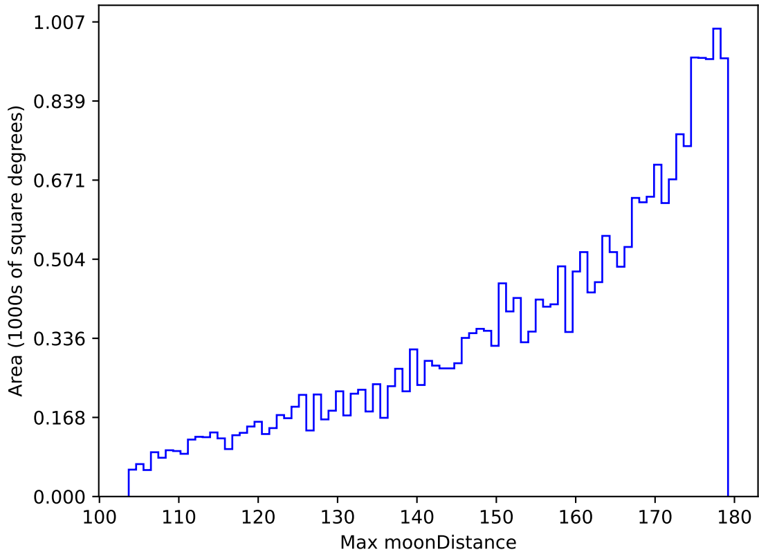
too_elab_r8_d2_giz_v3.4_10yrs All sky i band: Max moonDistance
