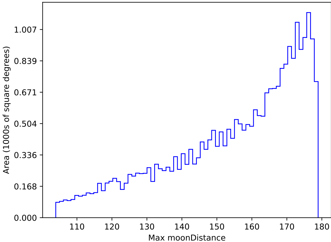
too_elab_r8_d2_giz_v3.4_10yrs All sky g band: Max moonDistance
