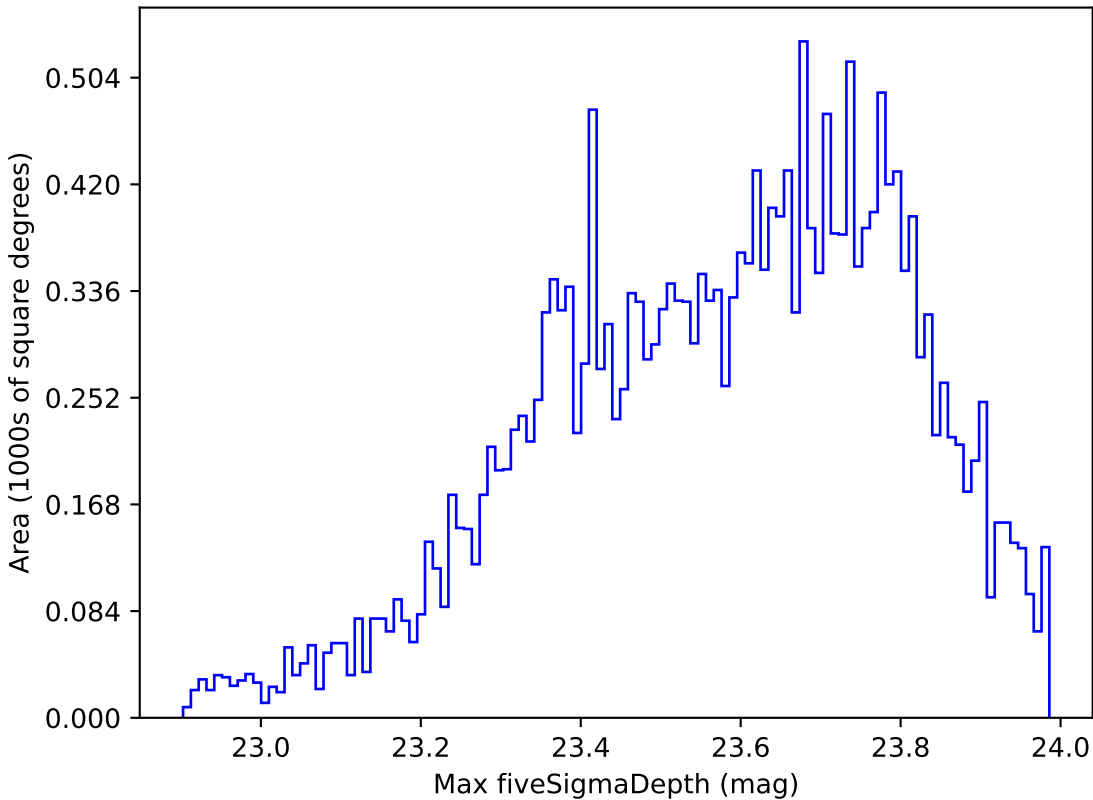
too_elab_r8_d2_giz_v3.4_10yrs Yr 1 u band: Max fiveSigmaDepth
