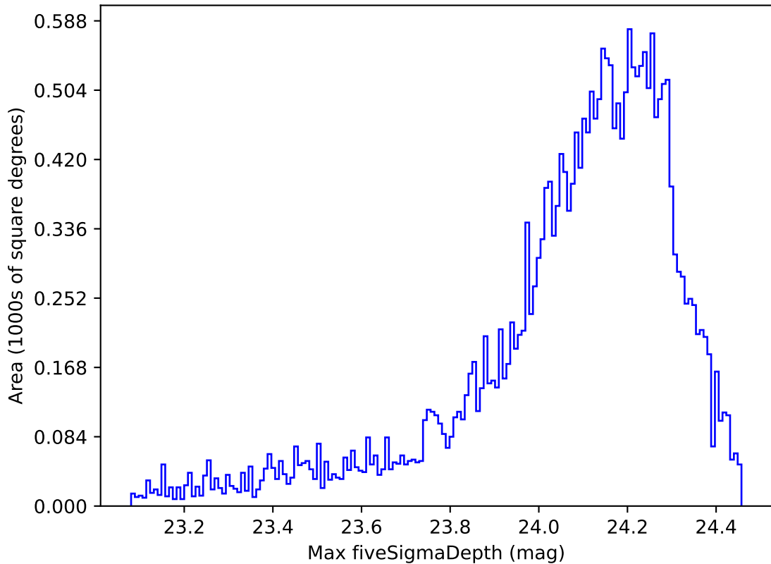
too_elab_r8_d2_giz_v3.4_10yrs Yr 1 i band: Max fiveSigmaDepth
