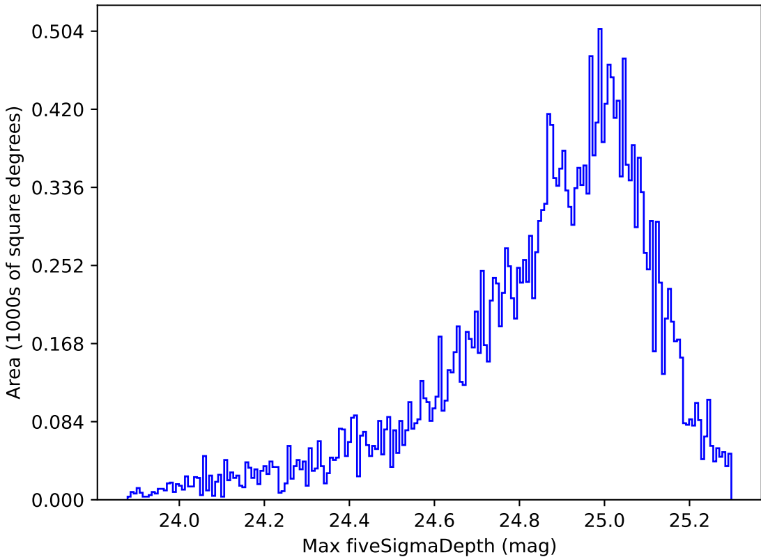
too_elab_r8_d2_giz_v3.4_10yrs Yr 1 all bands: Max fiveSigmaDepth
