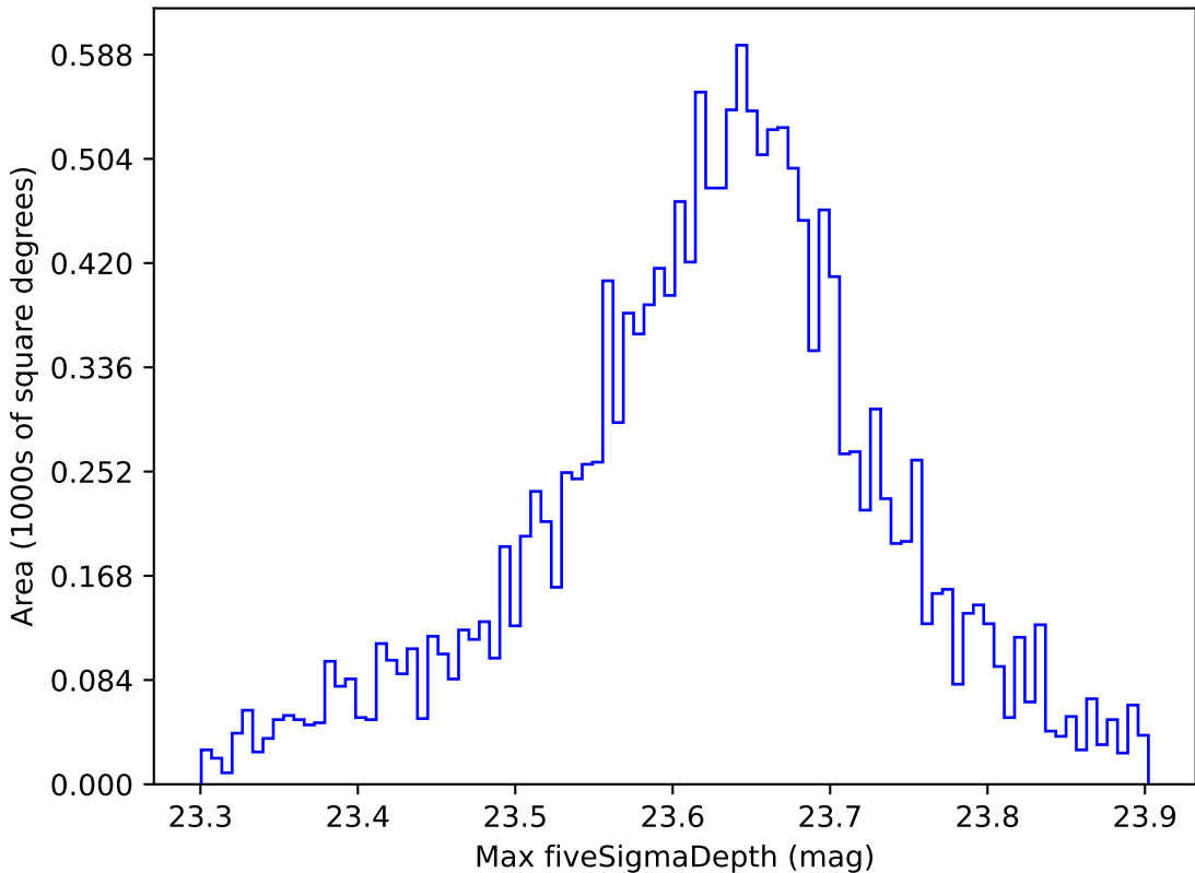
too_elab_r8_d2_giz_v3.4_10yrs WFD z band: Max fiveSigmaDepth
