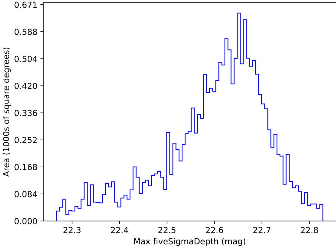
too_elab_r8_d2_giz_v3.4_10yrs WFD y band: Max fiveSigmaDepth
