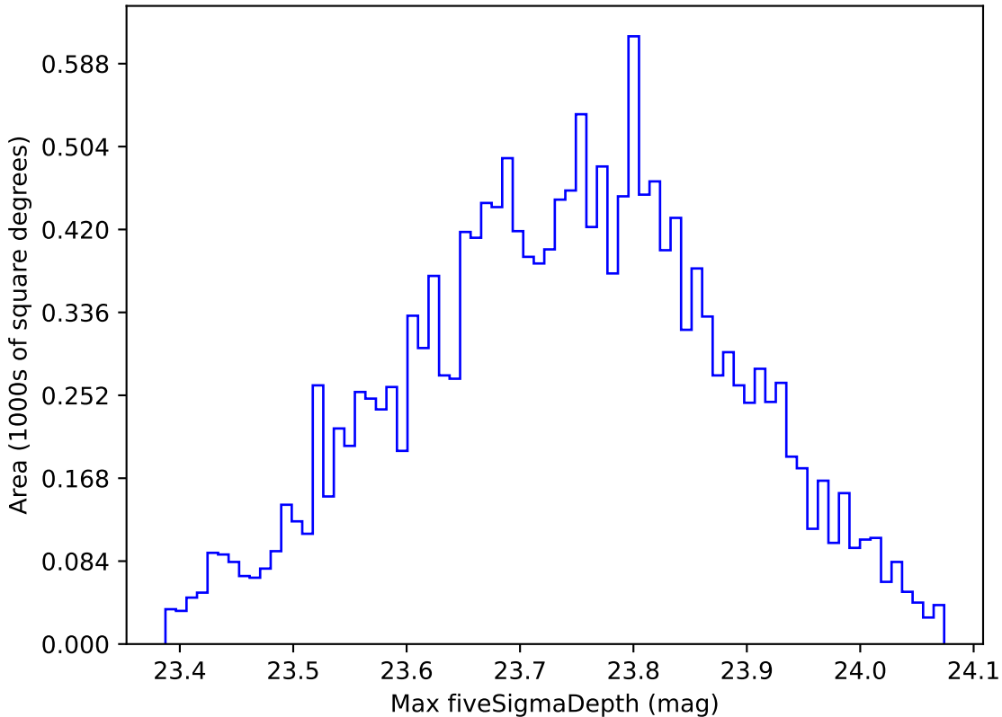
too_elab_r8_d2_giz_v3.4_10yrs WFD u band: Max fiveSigmaDepth
