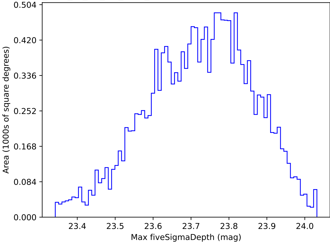
too_elab_r8_d2_giz_v3.4_10yrs WFD u band: Max fiveSigmaDepth
