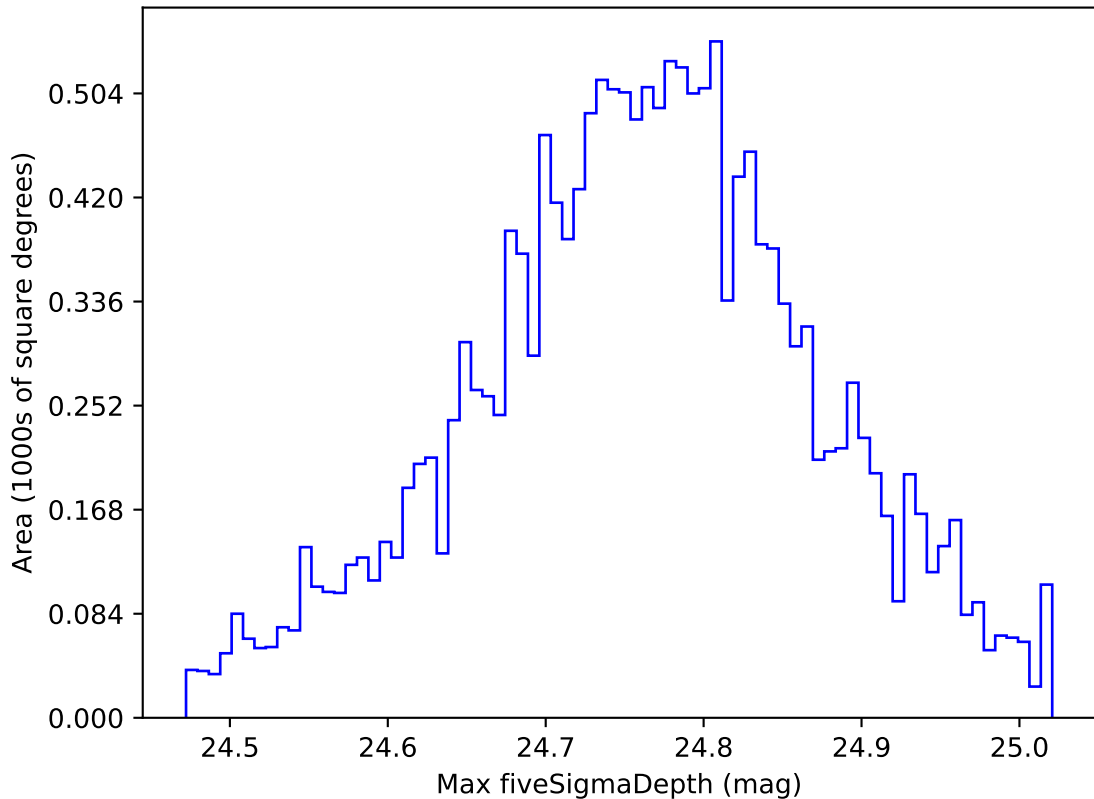
too_elab_r8_d2_giz_v3.4_10yrs WFD r band: Max fiveSigmaDepth
