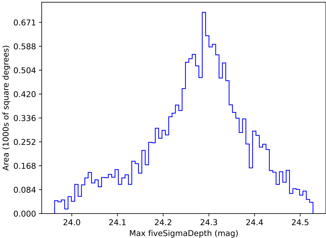
too_elab_r8_d2_giz_v3.4_10yrs WFD i band: Max fiveSigmaDepth
