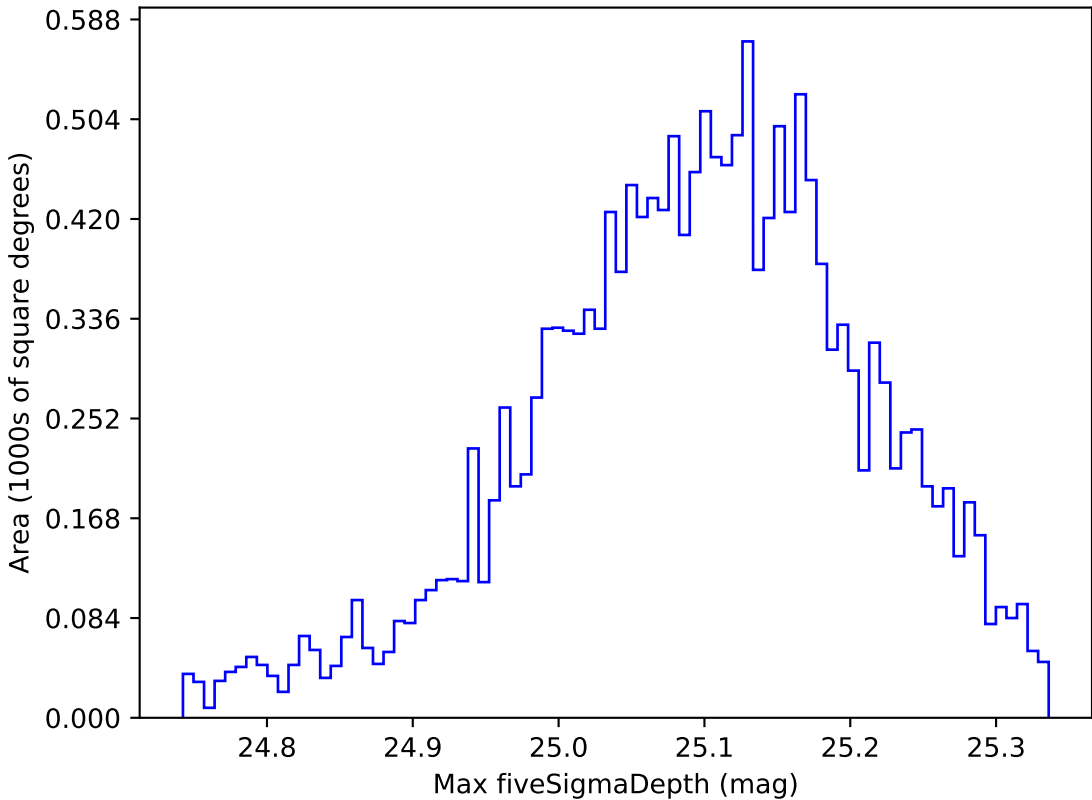
too_elab_r8_d2_giz_v3.4_10yrs WFD g band: Max fiveSigmaDepth
