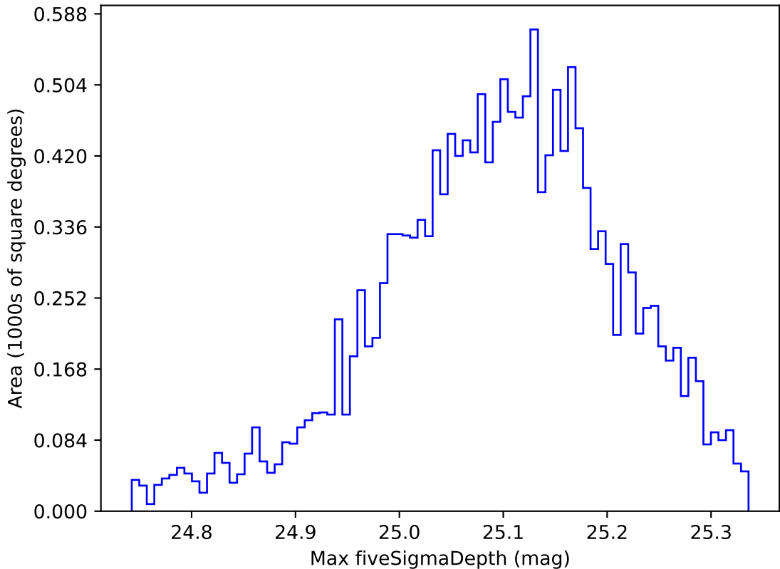
too_elab_r8_d2_giz_v3.4_10yrs WFD all bands: Max fiveSigmaDepth
