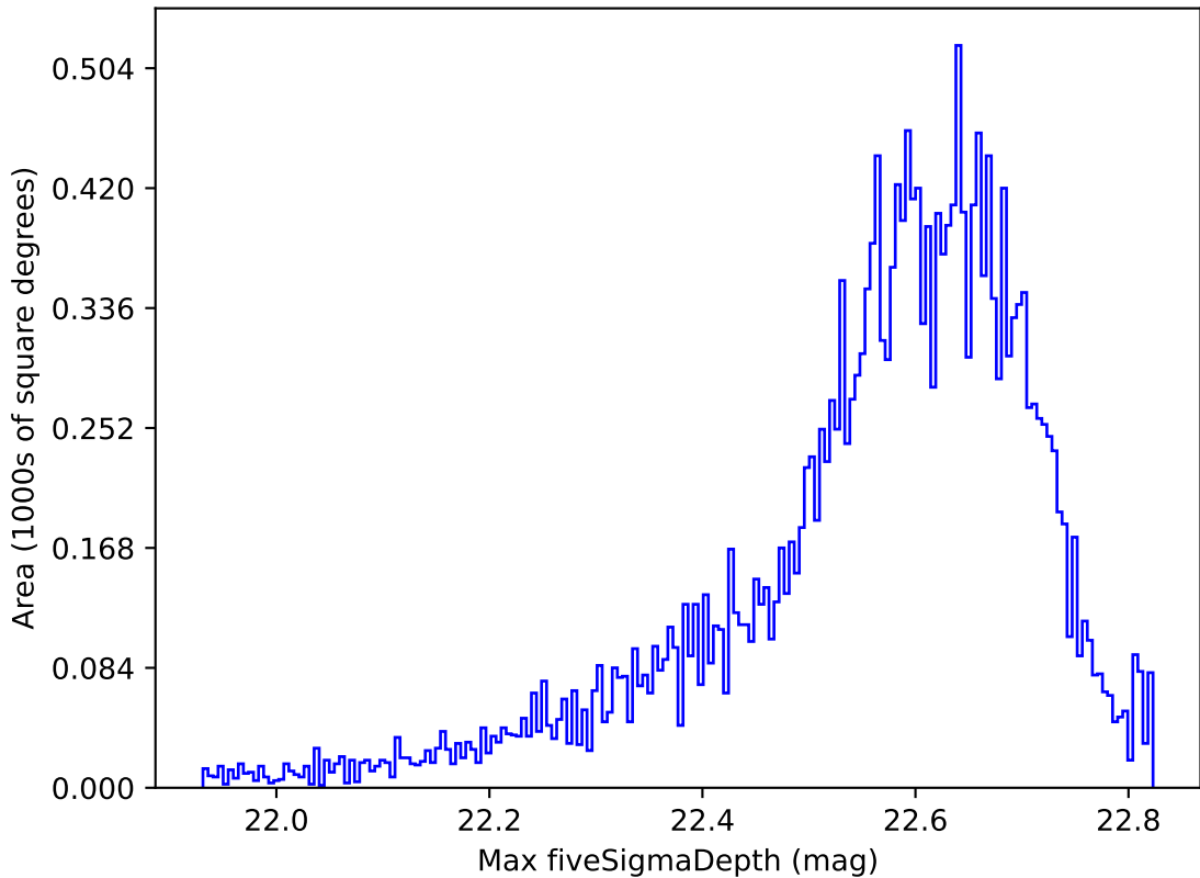
too_elab_r8_d2_giz_v3.4_10yrs All sky y band: Max fiveSigmaDepth
