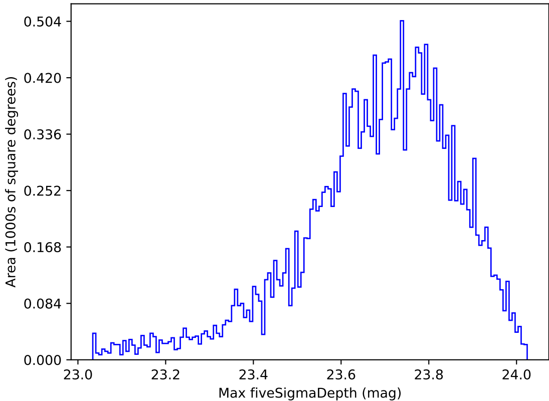
too_elab_r8_d2_giz_v3.4_10yrs All sky u band: Max fiveSigmaDepth
