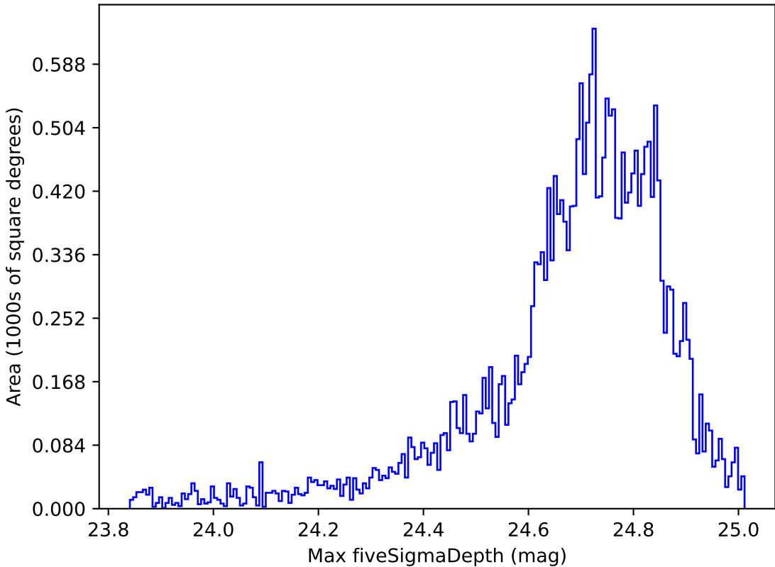
too_elab_r8_d2_giz_v3.4_10yrs All sky r band: Max fiveSigmaDepth
