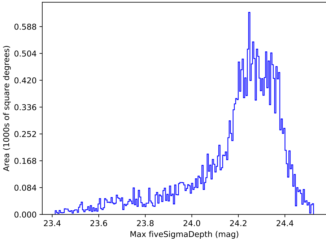
too_elab_r8_d2_giz_v3.4_10yrs All sky i band: Max fiveSigmaDepth
