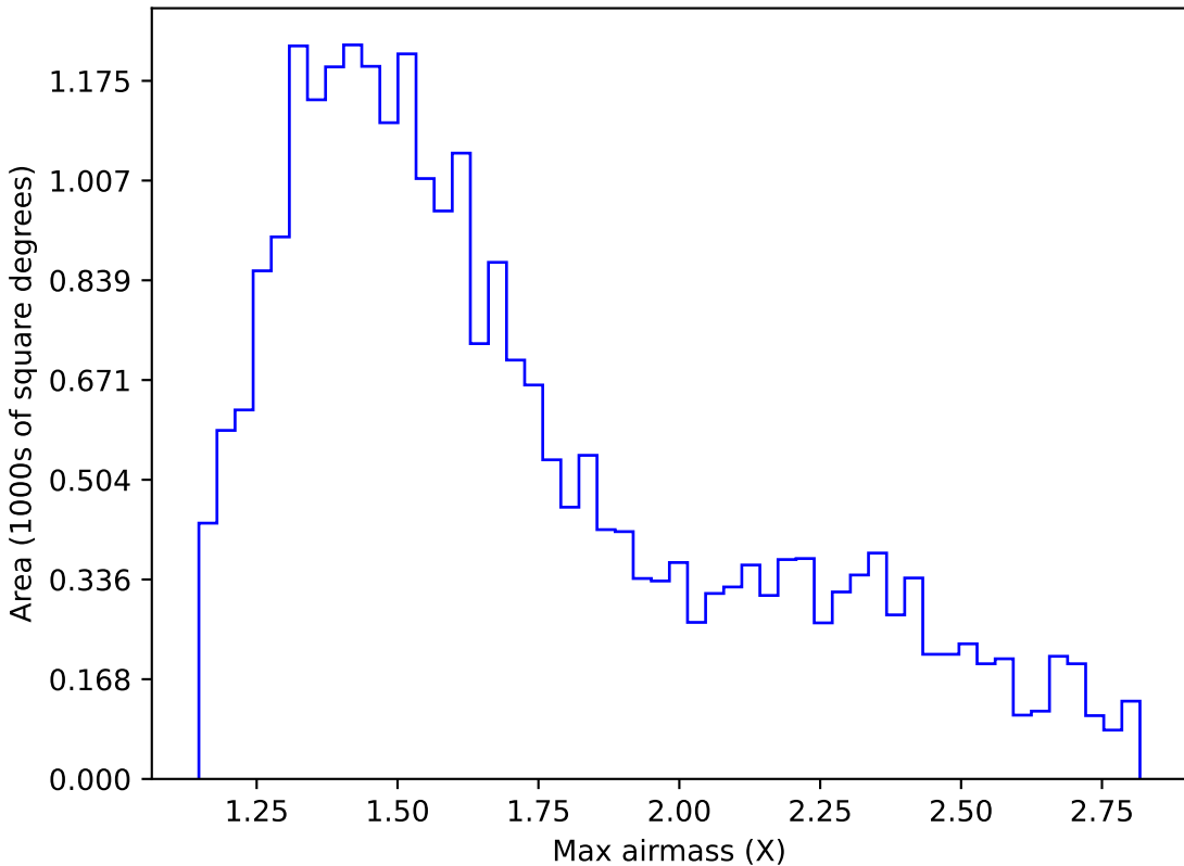
too_elab_r8_d2_giz_v3.4_10yrs Yr 1 z band: Max airmass
