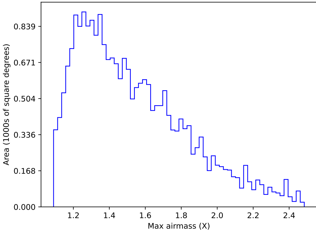
too_elab_r8_d2_giz_v3.4_10yrs Yr 1 u band: Max airmass
