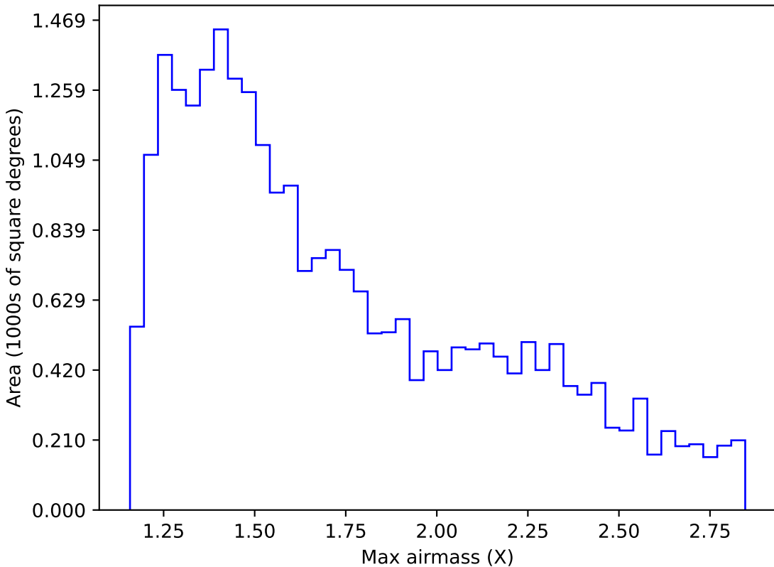
too_elab_r8_d2_giz_v3.4_10yrs Yr 1 i band: Max airmass
