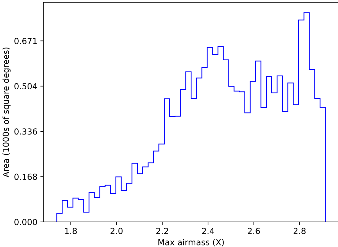
too_elab_r8_d2_giz_v3.4_10yrs WFD z band: Max airmass
