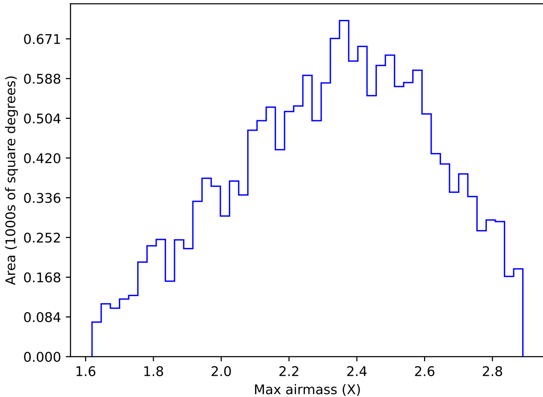
too_elab_r8_d2_giz_v3.4_10yrs WFD y band: Max airmass
