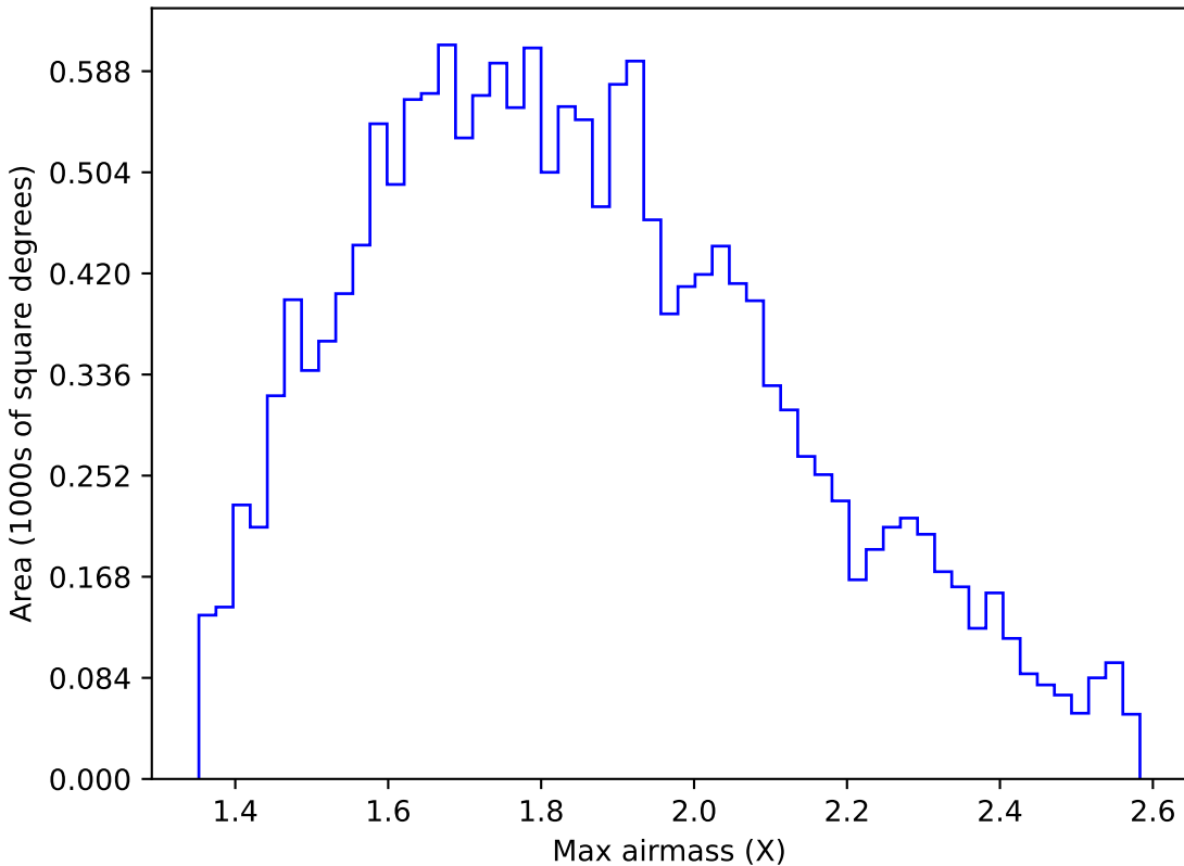
too_elab_r8_d2_giz_v3.4_10yrs WFD u band: Max airmass
