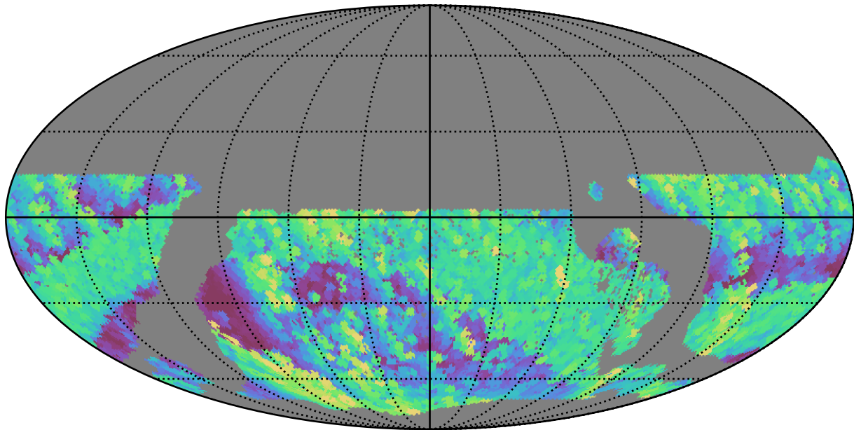
too_elab_r8_d2_giz_v3.4_10yrs WFD r band: Max airmass
