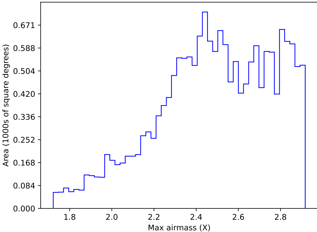
too_elab_r8_d2_giz_v3.4_10yrs WFD i band: Max airmass
