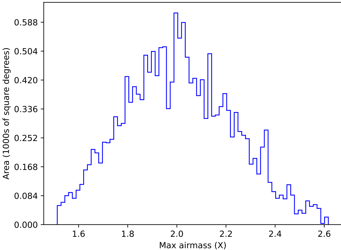
too_elab_r8_d2_giz_v3.4_10yrs WFD g band: Max airmass
