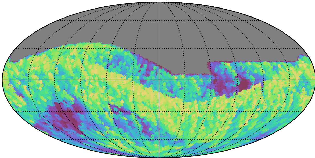
too_elab_r8_d2_giz_v3.4_10yrs All sky z band: Max airmass
