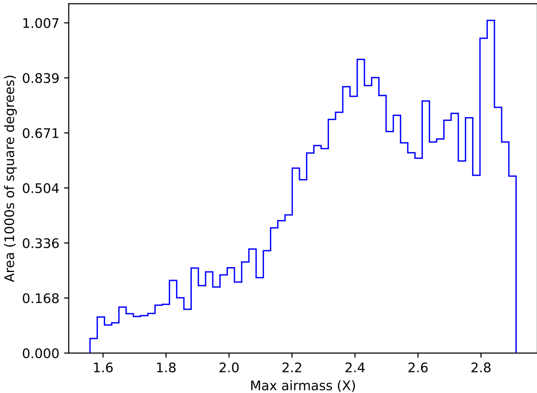
too_elab_r8_d2_giz_v3.4_10yrs All sky z band: Max airmass
