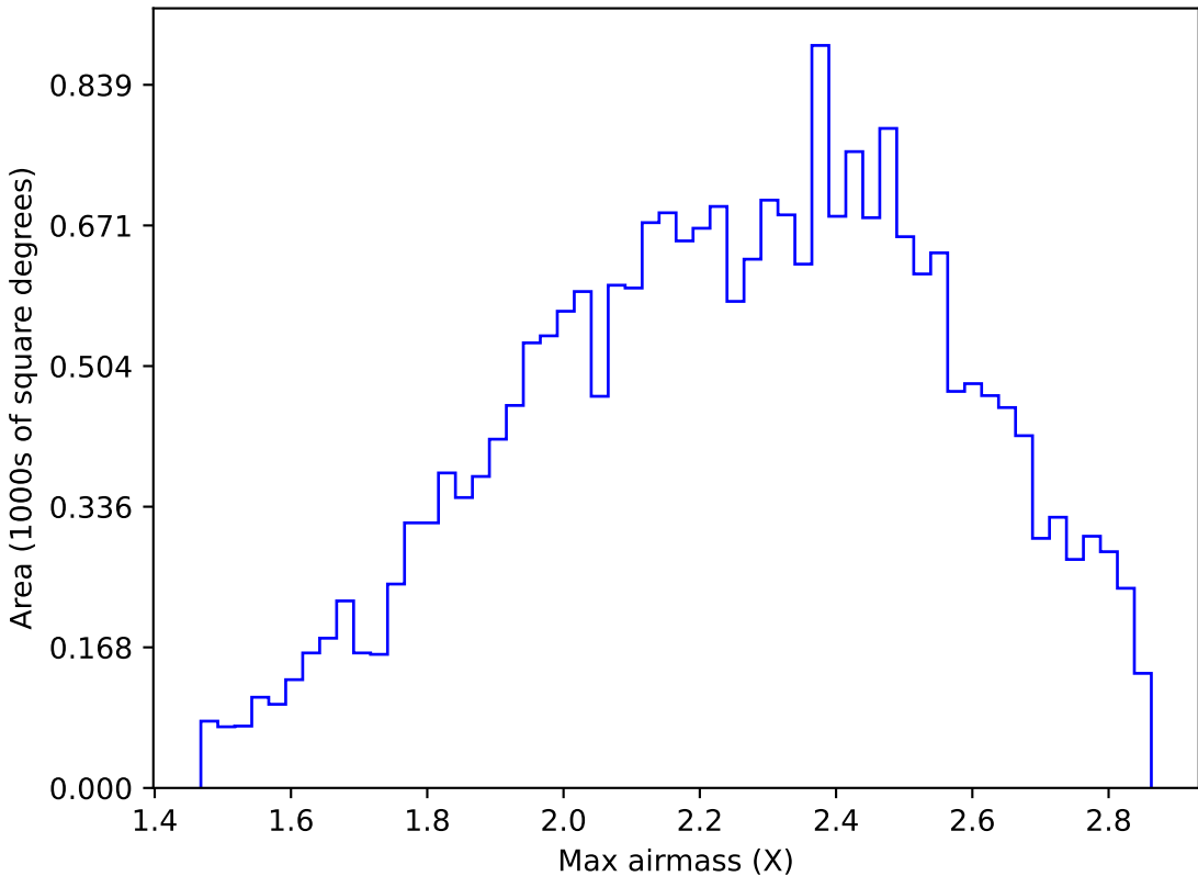
too_elab_r8_d2_giz_v3.4_10yrs All sky y band: Max airmass
