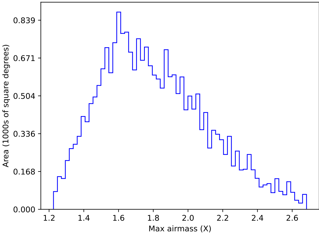
too_elab_r8_d2_giz_v3.4_10yrs All sky u band: Max airmass
