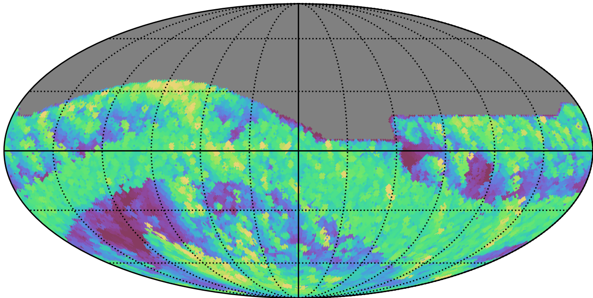
too_elab_r8_d2_giz_v3.4_10yrs All sky r band: Max airmass
