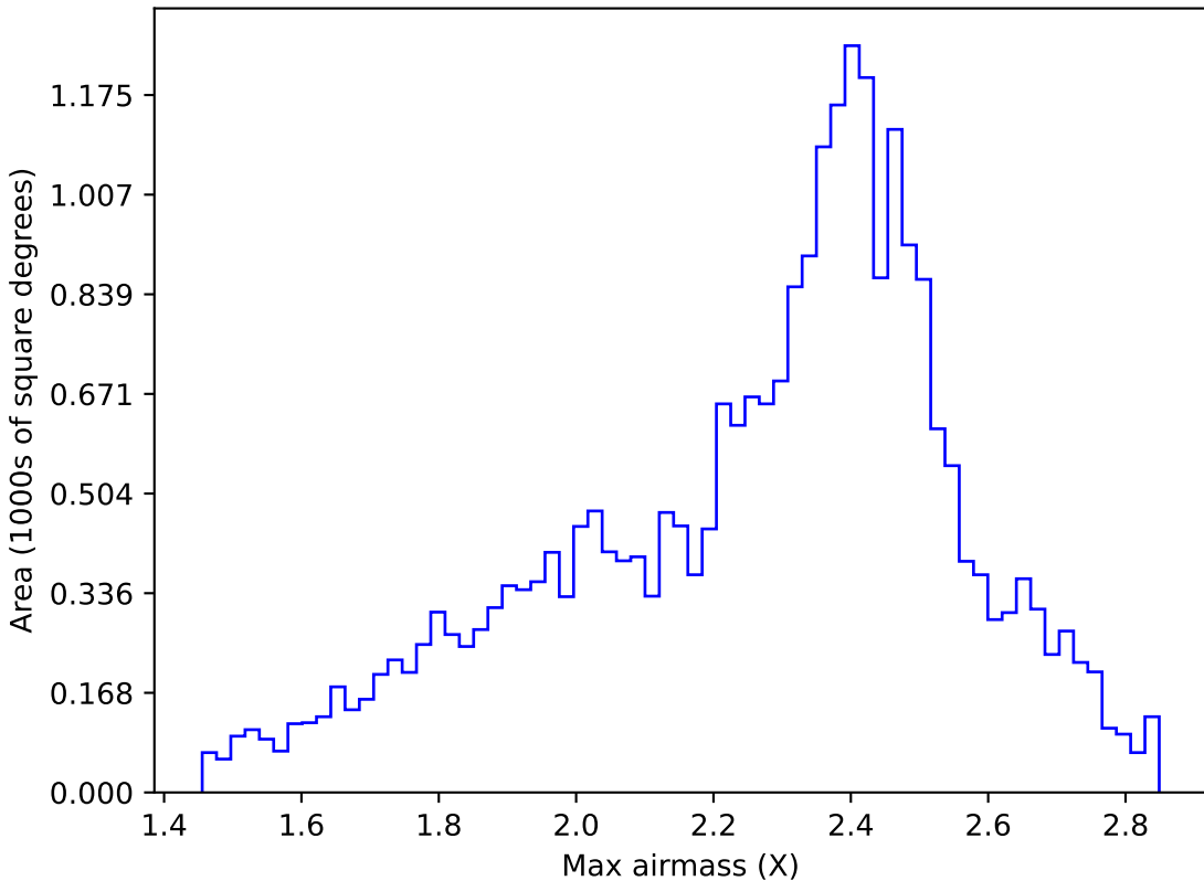
too_elab_r8_d2_giz_v3.4_10yrs All sky r band: Max airmass
