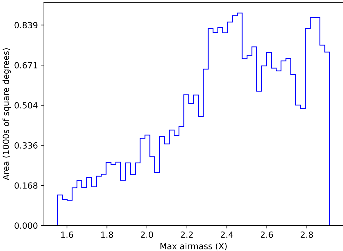
too_elab_r8_d2_giz_v3.4_10yrs All sky i band: Max airmass
