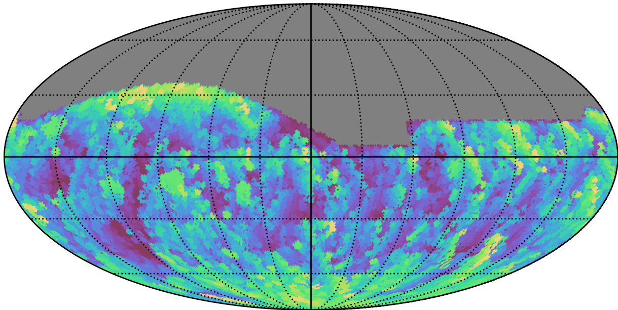
too_elab_r8_d2_giz_v3.4_10yrs All sky g band: Max airmass
