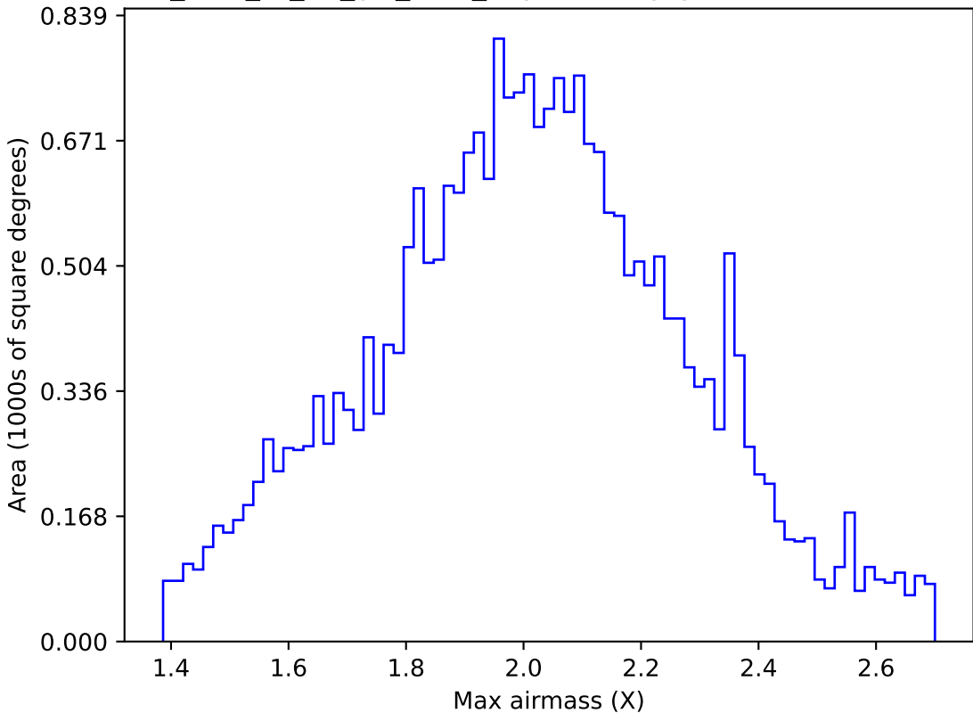
too_elab_r8_d2_giz_v3.4_10yrs All sky g band: Max airmass
