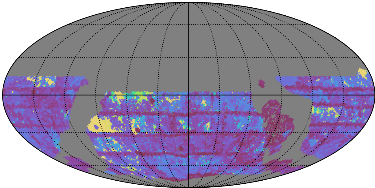
too_elab_r8_d2_giz_v3.4_10yrs WFD z band: Max Inter-Night Gap
