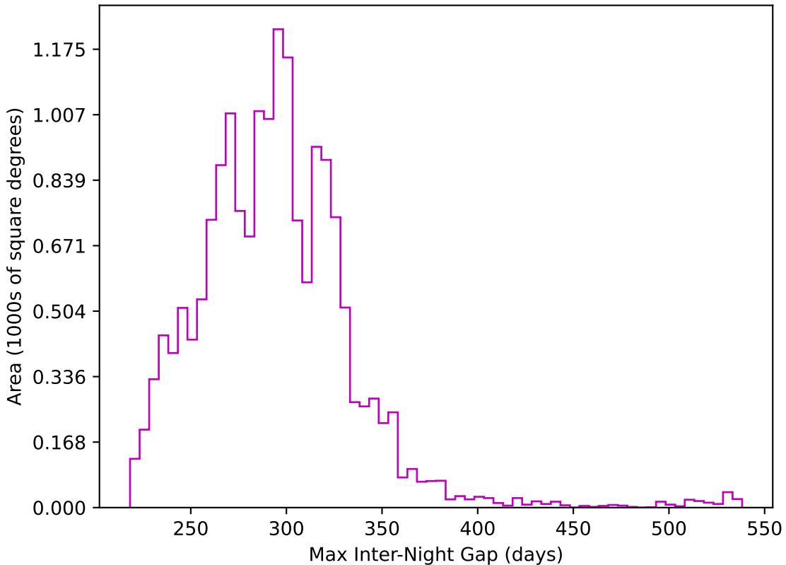
too_elab_r8_d2_giz_v3.4_10yrs WFD z band: Max Inter-Night Gap
