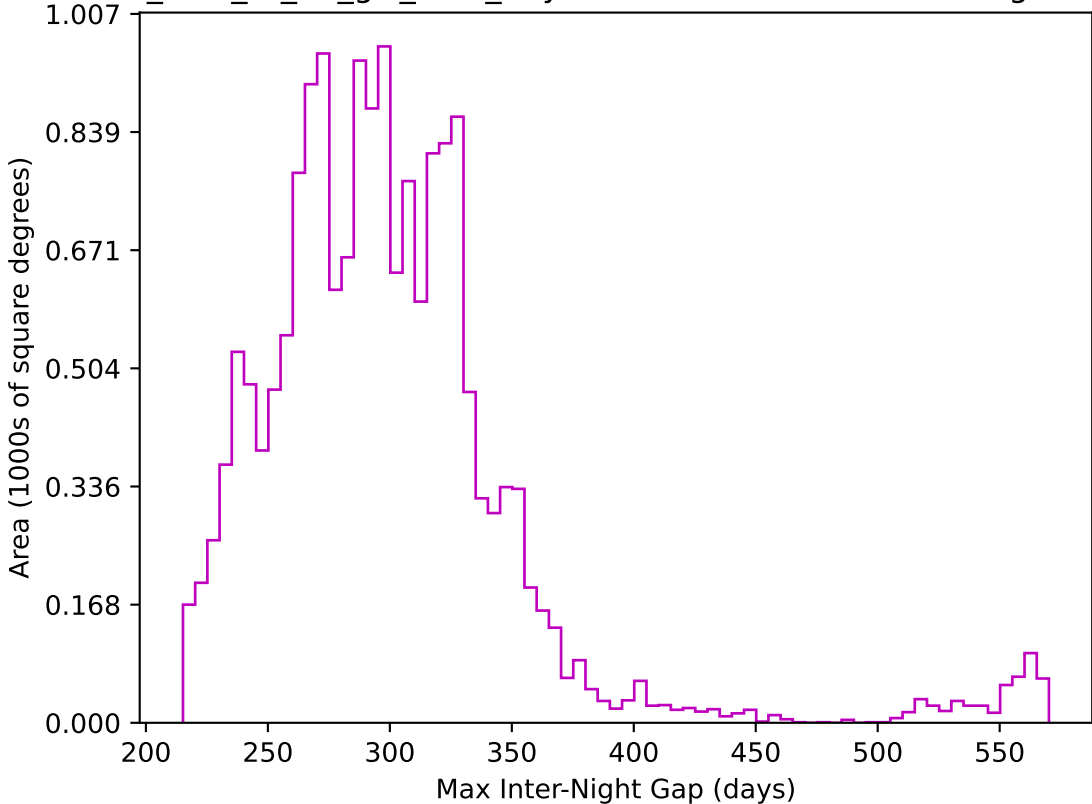
too_elab_r8_d2_giz_v3.4_10yrs WFD z band: Max Inter-Night Gap
