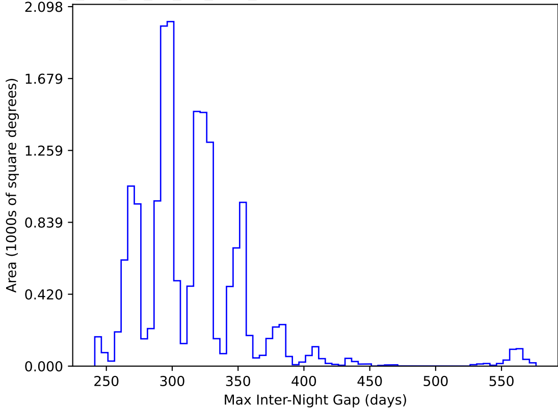
too_elab_r8_d2_giz_v3.4_10yrs WFD y band: Max Inter-Night Gap
