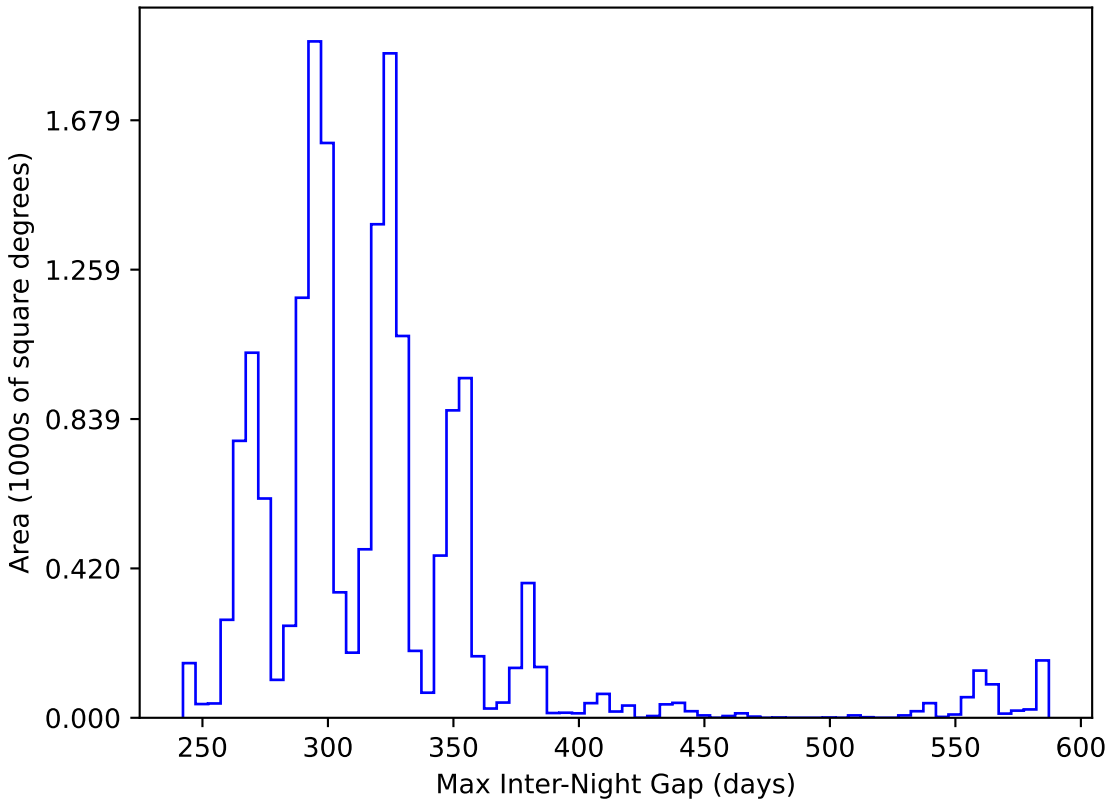
too_elab_r8_d2_giz_v3.4_10yrs WFD y band: Max Inter-Night Gap
