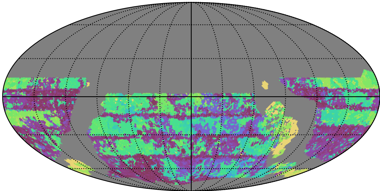
too_elab_r8_d2_giz_v3.4_10yrs WFD u band: Max Inter-Night Gap
