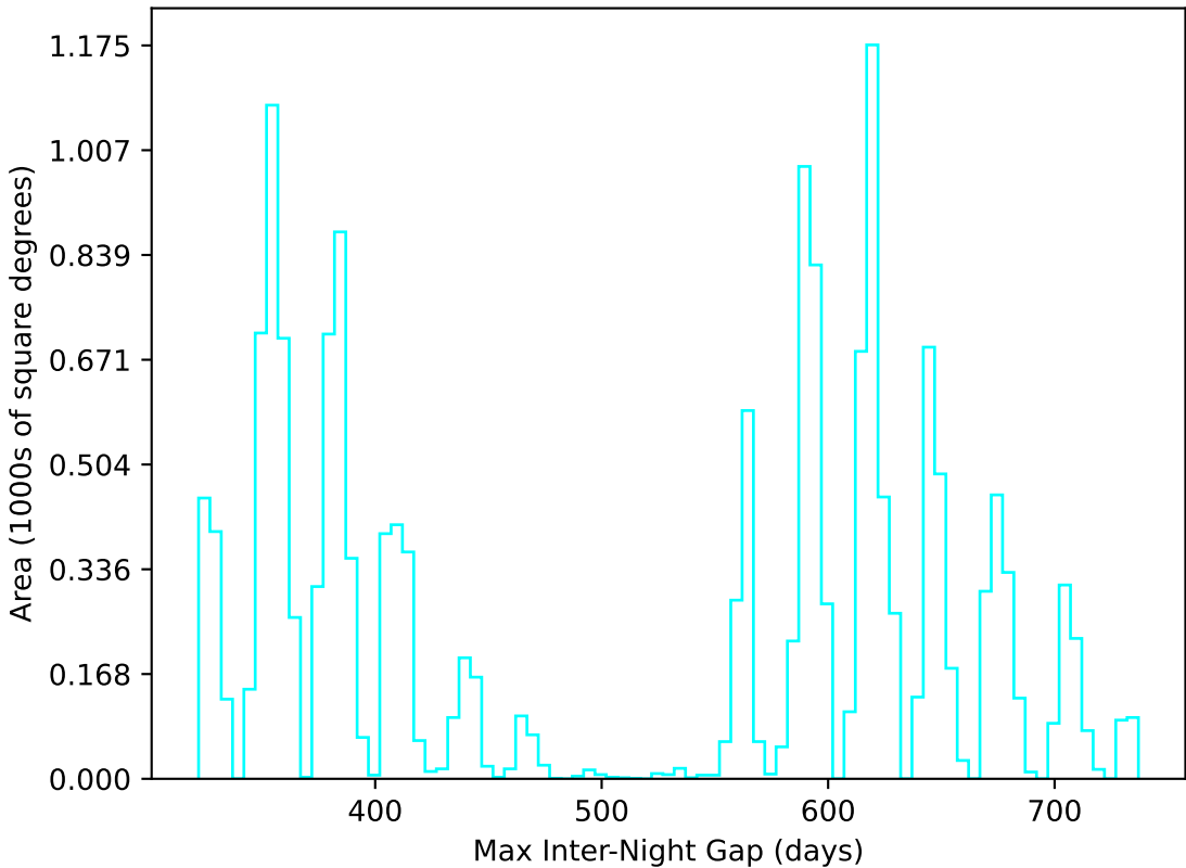
too_elab_r8_d2_giz_v3.4_10yrs WFD u band: Max Inter-Night Gap
