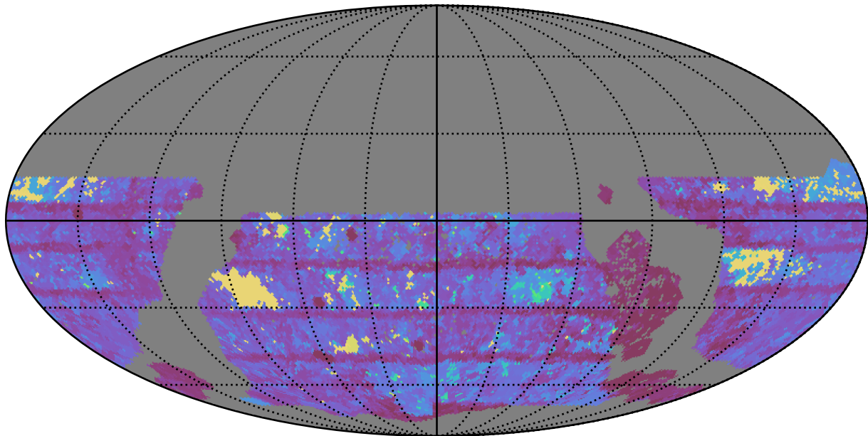
too_elab_r8_d2_giz_v3.4_10yrs WFD r band: Max Inter-Night Gap
