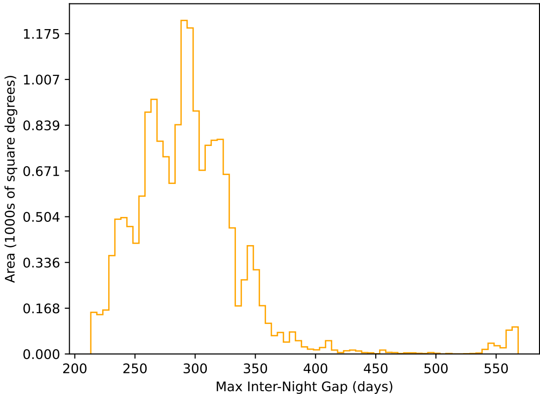
too_elab_r8_d2_giz_v3.4_10yrs WFD r band: Max Inter-Night Gap
